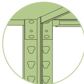
T Upright Post is 2" wide with 2 rows of keyhole slots.
