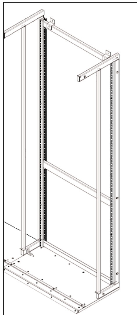
Frame Weldment
