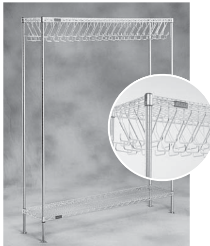
hooks on 1 1/2" (38mm) centers on all four shelf sides
